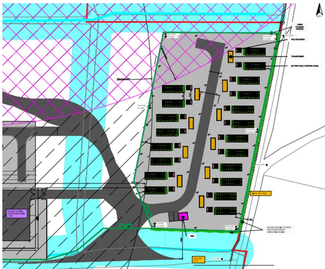
Figure 2 – Site layout plan 3
